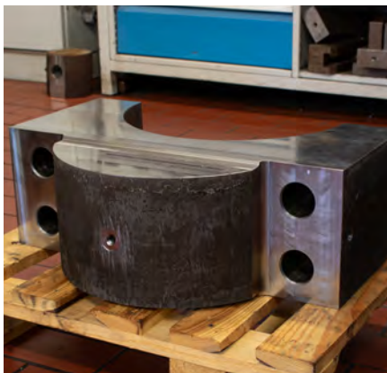
Pleuel Schale
